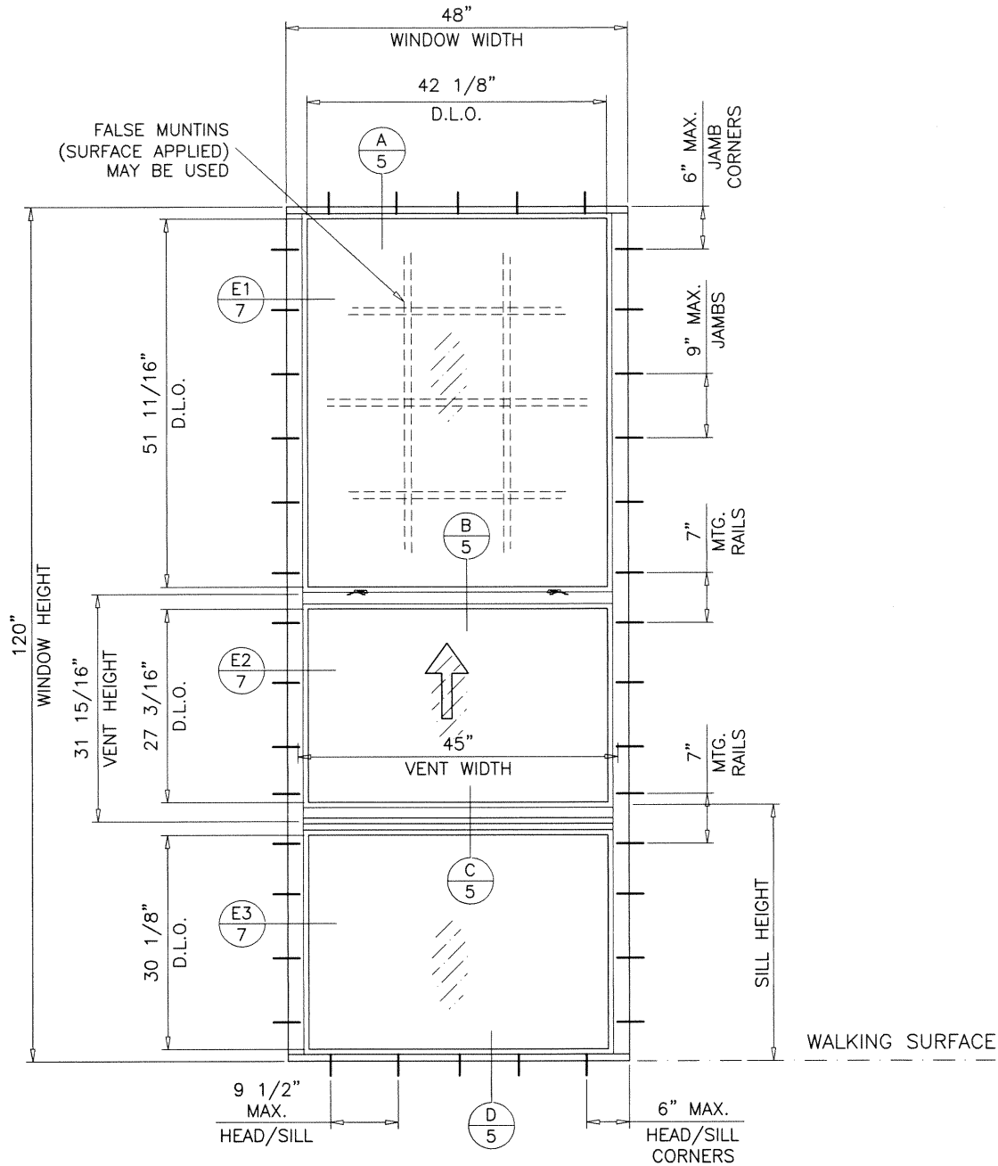
TYPICAL ELEVATION
